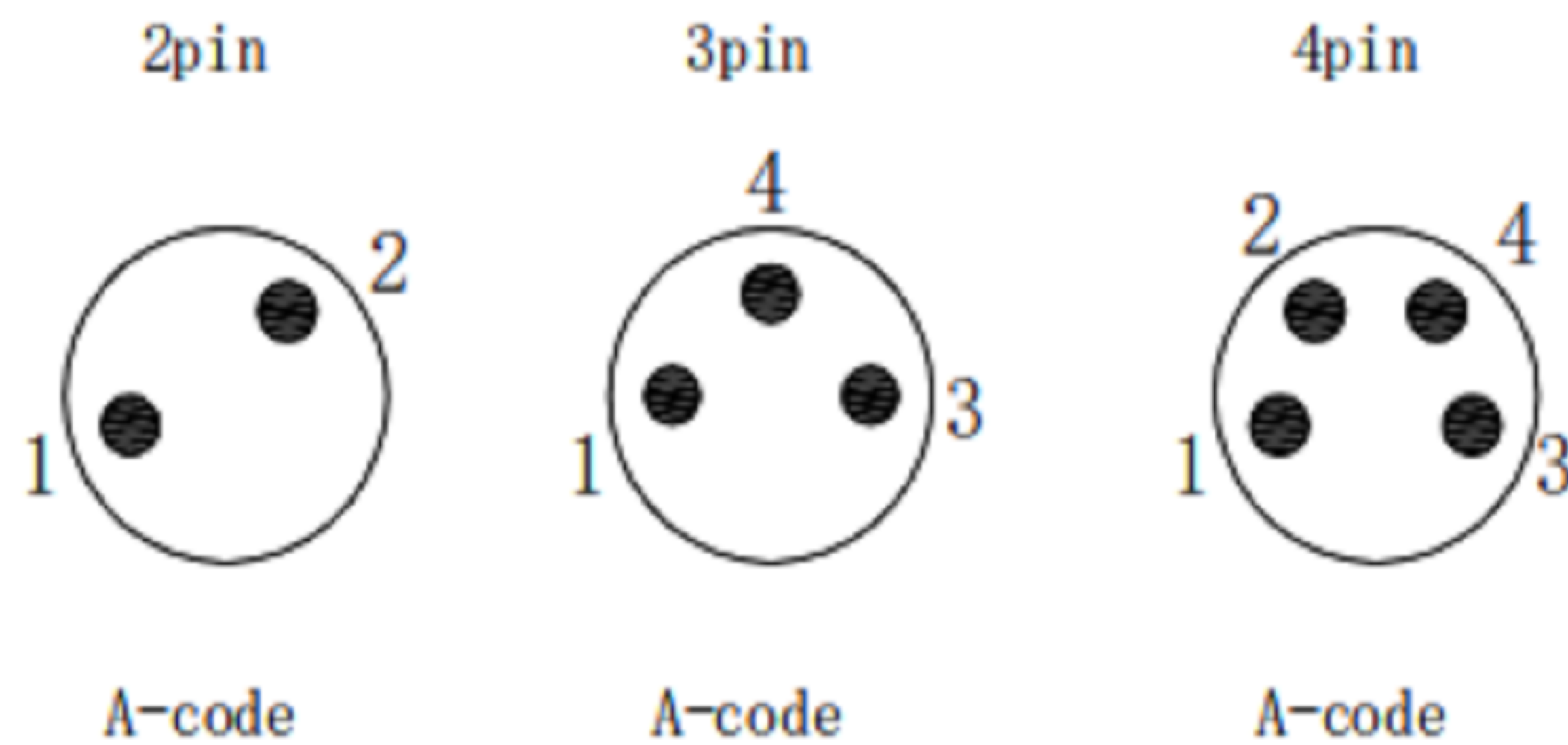
Pin assignment front view/针位分布前视图
